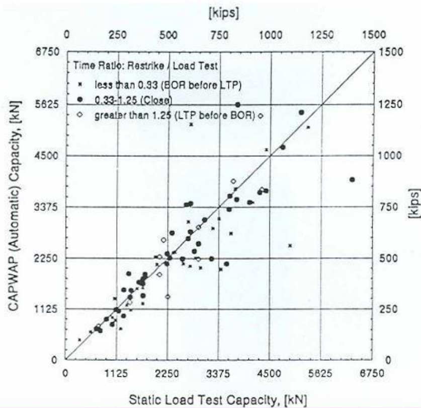
Figure 1(a): CAPWAP (Automatic) Capacity vs Static Load Test Capacity Showing Different Time Ratios
