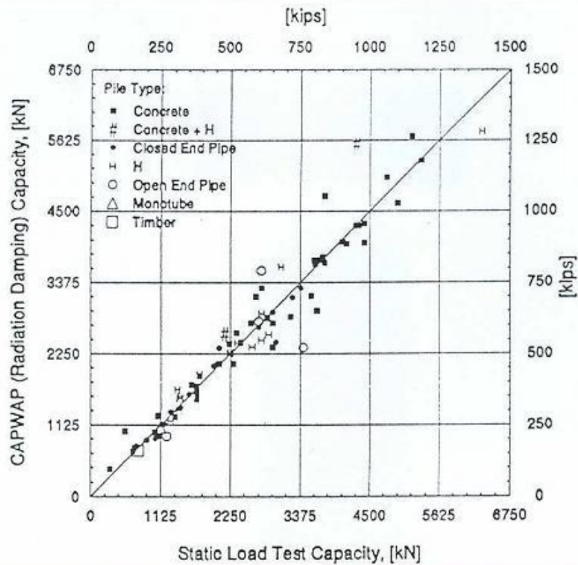
Figure 6: CAPWAP (Radiation Damping) Capacity vs Static Load Test Capacity Showing Different Pile Types
