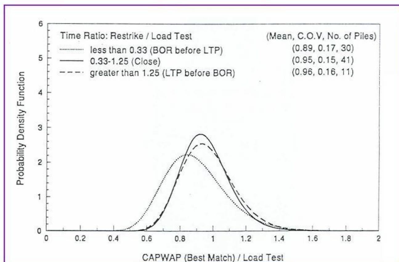
Figure 2(b): Log-Normal Probability Density Function for CAPWAP (Best Match) Capacity Prediction at Different Time Ratios
